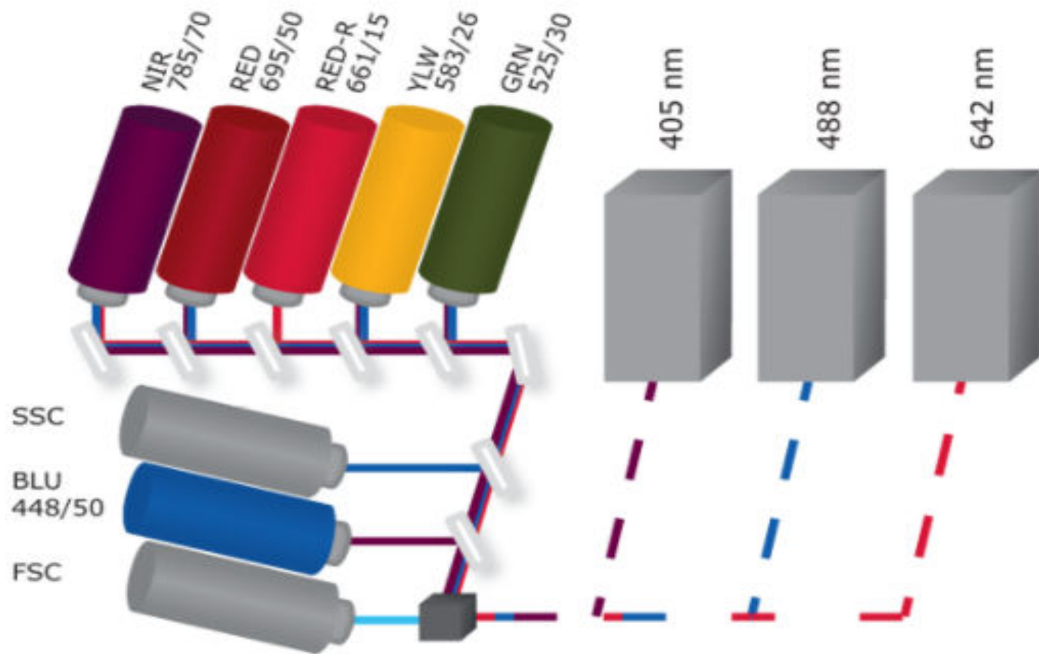
Optical layout for the easyCyte 12 three-laser system
